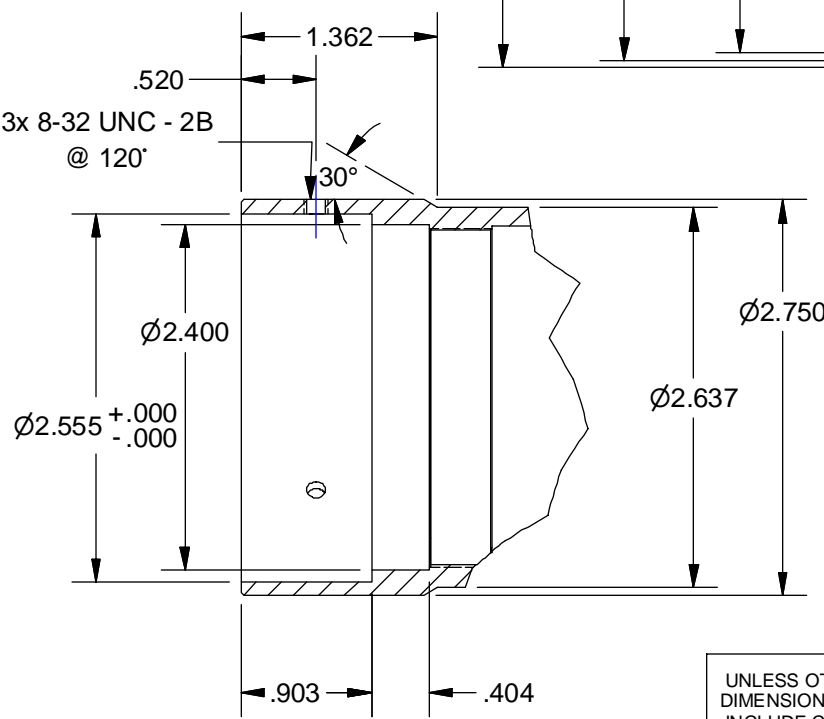
DETAIL CUSTOM FIT INTERFACE SCALE 3 / 4
